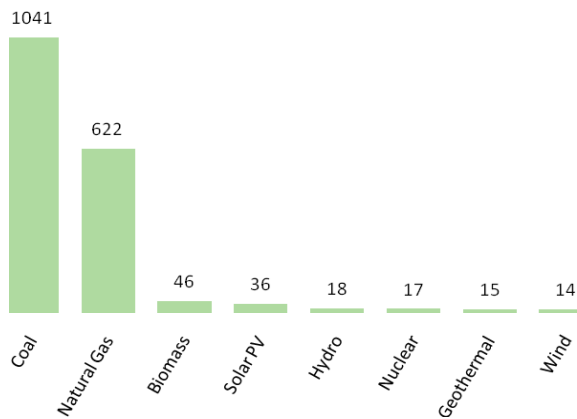
Nuclear Energy’s Low Carbon Footprint (in tons of CO2 equivalent per gigawatt-hour) Source: Nuclear Energy Institute. “Nuclear Energy Plays Essential Role in Climate Change Initiatives”. Policy Brief, September 2009.
